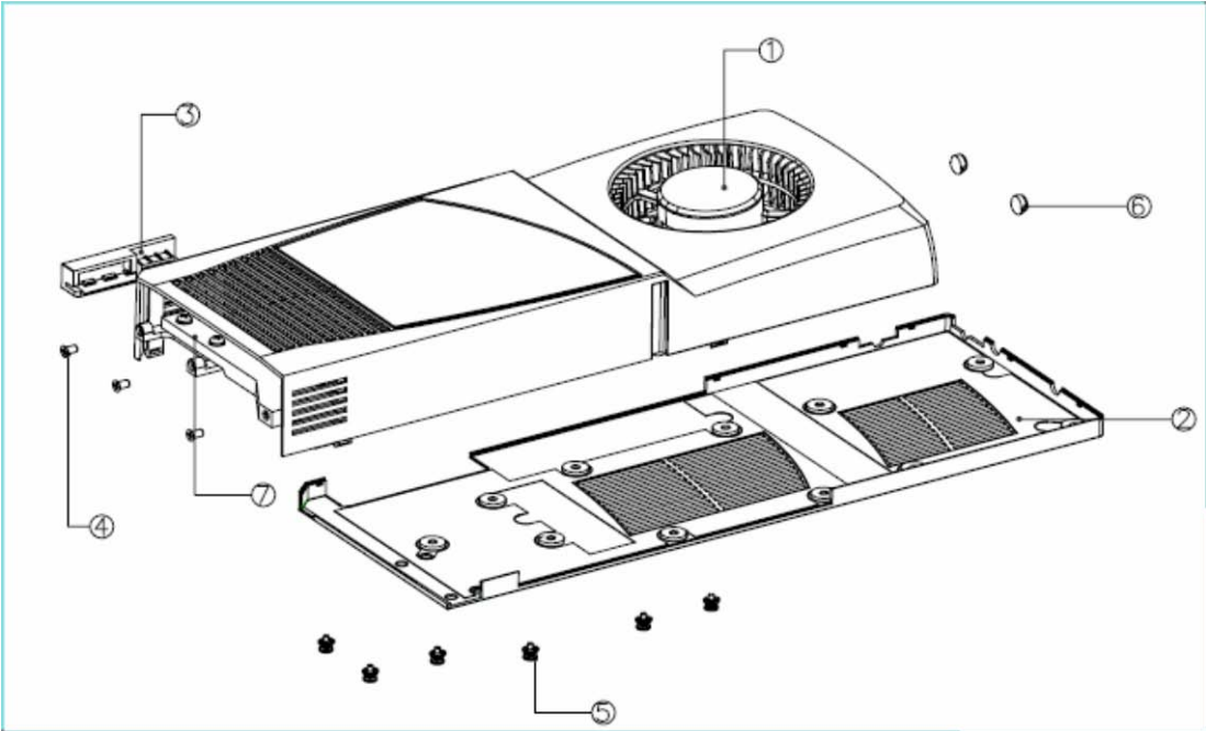
Figure 7. TM72 Active Fan Sink
