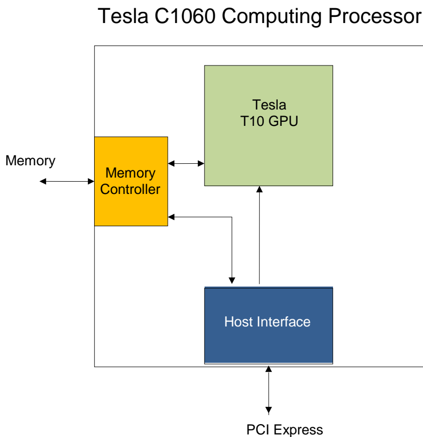
Figure 1. Tesla C1060 Block Diagram
