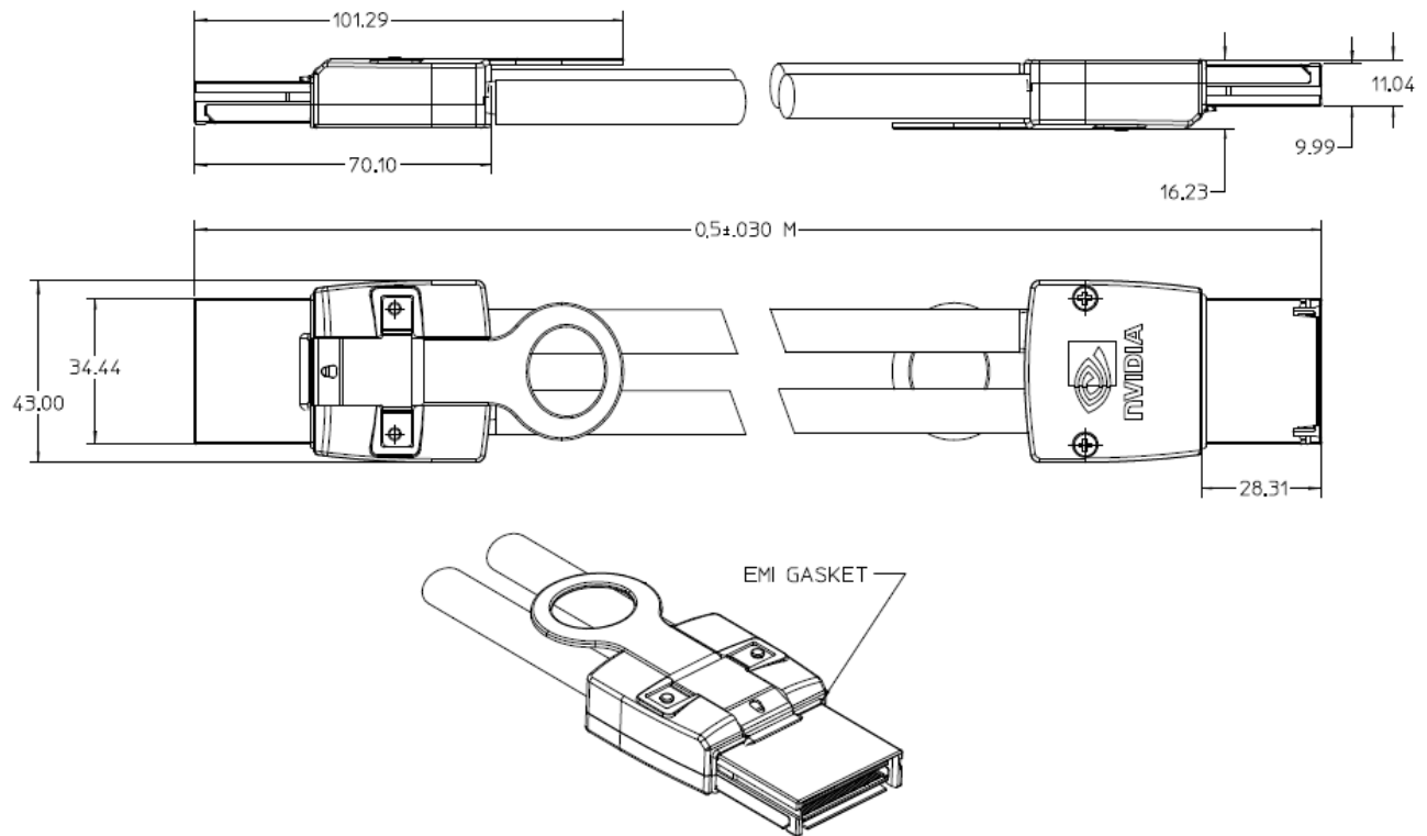
Figure 4. PCI Express Cable
