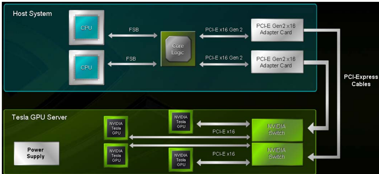
Figure 1. Tesla S870 GPU Computing System Architecture
