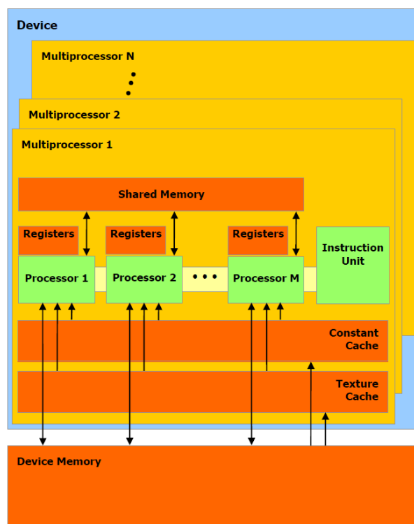
Fig. 2. G80 architecture. On the 8800GTX, there are sixteen multiprocessors, each containing eight stream processors, for a total of 128 processors. The stream processors within a multiprocessor share an instruction unit, so maximum parallelism is obtained when only when the stream processors execute the same instruction stream (potentially on different data). Source: NVIDIA CUDA 0.8 SDK.
