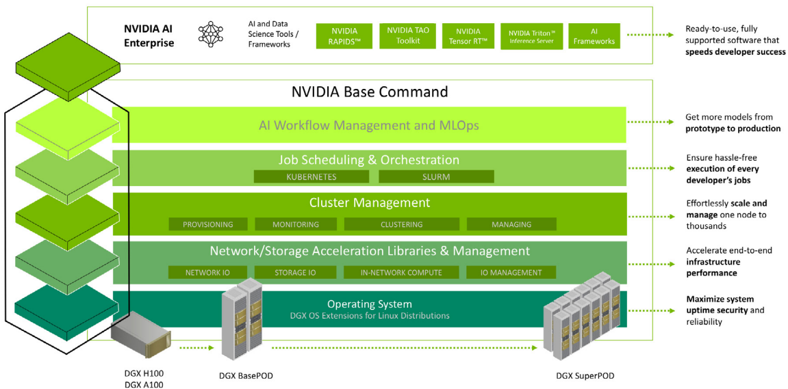
NVIDIA Base Command Software Stack
